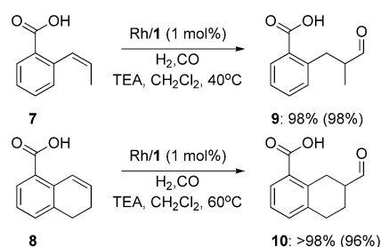
Scheme 4. Hydroformylation of \beta -substituted vinyl arenes 7 and 8 with the supramolecular catalyst Rh/ 1 . Product yield determined by NMR analysis of the reaction mixture; no side products were observed. Value within parentheses indicates yield of isolated product for reactions conducted on a 0.5–0.8 mmol scale.
