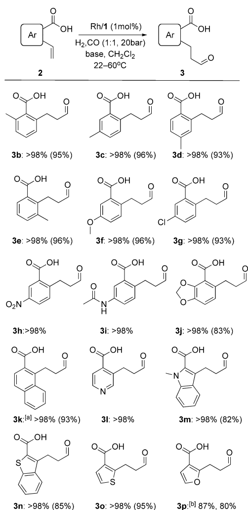
Scheme 3. Hydroformylation of vinyl 2-carboxyarenes 2 with the Rh/ 1 catalyst. Product yield and selectivity determined by ^1\text{H} and ^{13}\text{C} NMR analysis of the reaction mixture. Value within parentheses indicates yield of isolated product for reactions conducted on a 0.3–0.8 mmol scale. Full conversion of the starting material in all cases (except where noted). Reagents and conditions: [ 2 ] = 0.2 M, base = DIPEA or TEA (0.5–1.5 equiv), [\text{Rh}(\text{CO})_2(\text{acac})] (1 mol%), ligand 1 (1.1 mol%), \text{CO}/\text{H}_2 = 1:1 (20 bar), 22–60°C, 24–72 h. [a] 95% conversion. [b] Regioselectivity toward aldehyde 3p and chemoselectivity towards aldehydes, respectively. For full experimental details see the Supporting Information. TEA = triethylamine.
